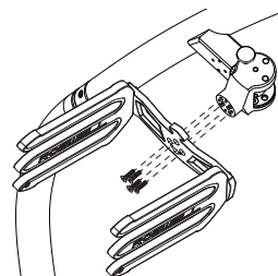
Swivel Tower Mount
