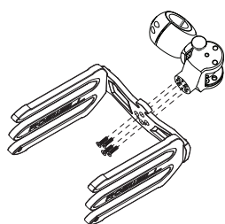
Swivel & Clamp
