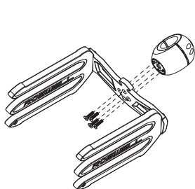
Universal Clamp
