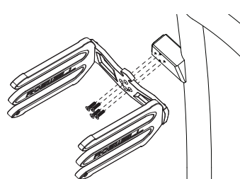
Fixed Tower Mount
